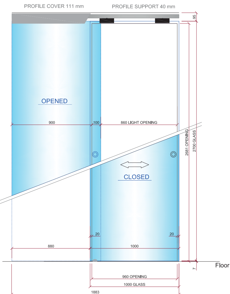
LINTEL MOUNTING SYSTEM B
