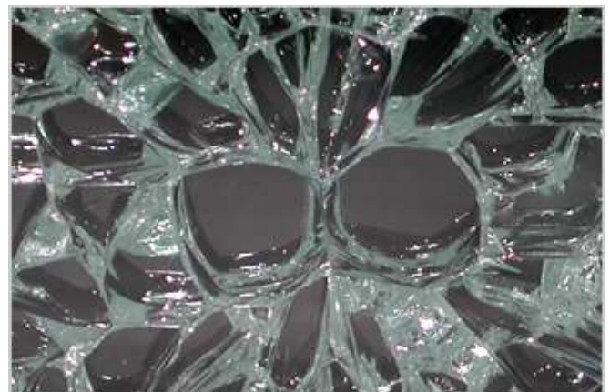
Typical breakage starting from a NiS inclusion
