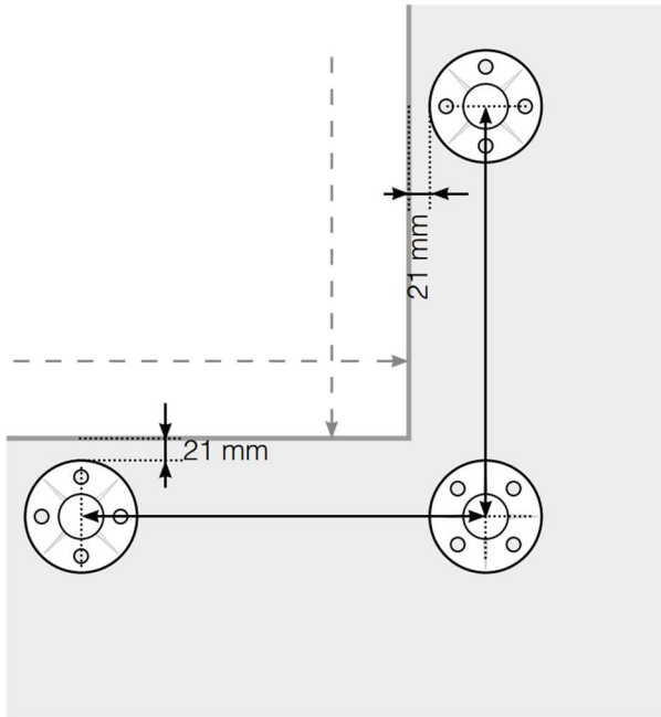
Inside corner 90°
